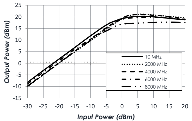
Pin vs. Pout, VDD = +5V
